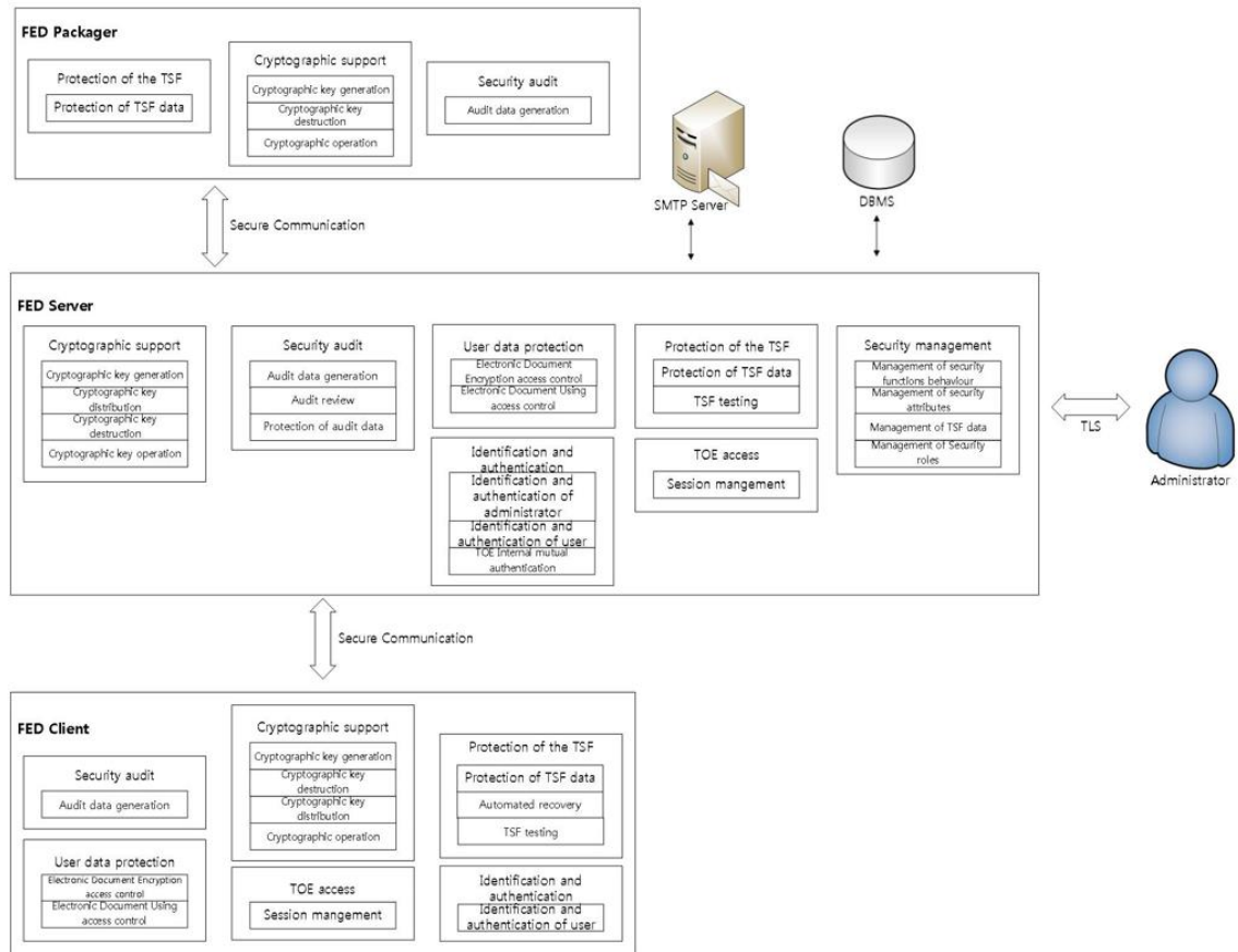
[Figure 2] TOE Logical scope
